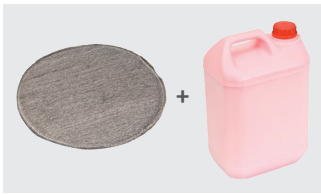
Crystallization
