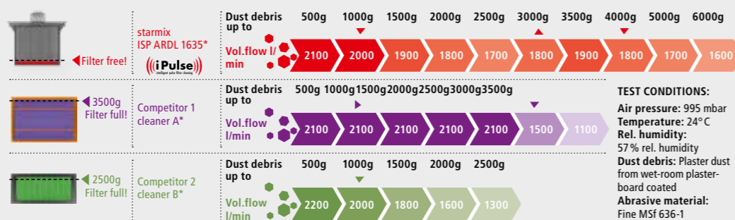
Fill level/volume flow comparison with plasterboard
