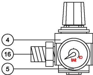
High flow regulator
