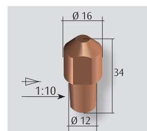
Electrode for lower arm in pressed-in electrode version
