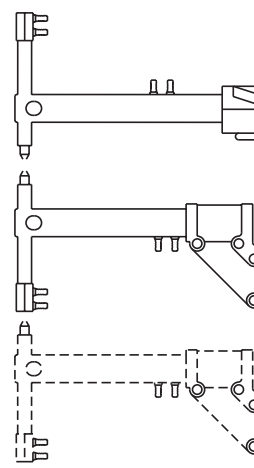
Lower arm with adjustable height
