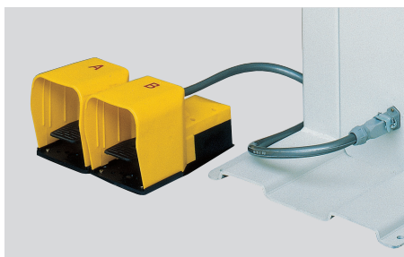
Possibility of a two-step pedal: squeeze without welding and welding after pressing the second step
