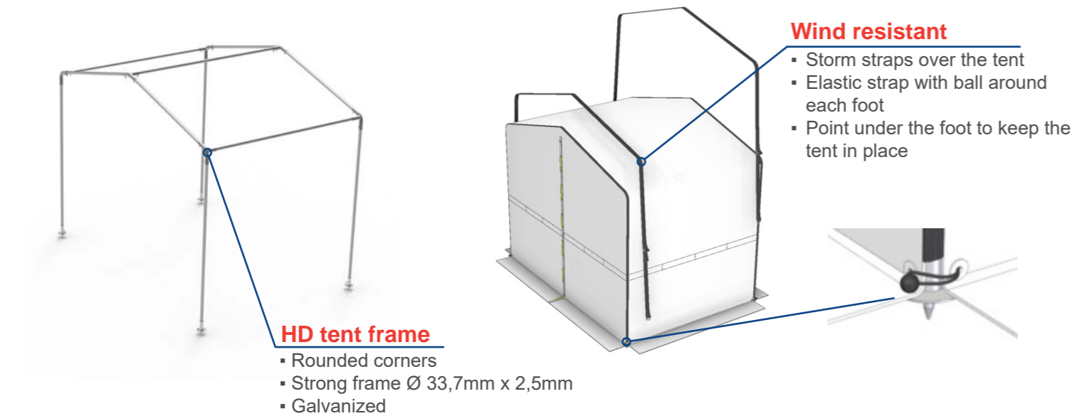
HD welding /working tent (example) with 2 roofcovers interconnected with water-repellent zippers
