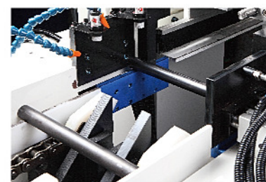
Length Measuring ( LM-3000 )
