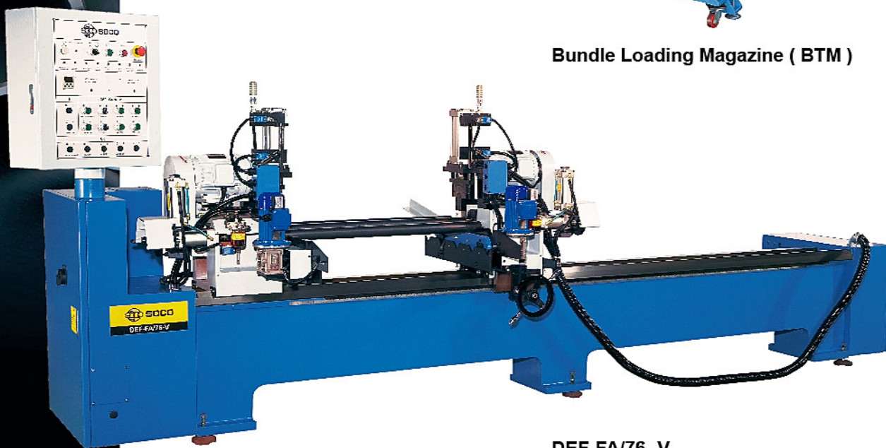
DEF-FA/76- V Double Tube Ends Chamfering with Long Working Lengths from 200mm ~ 3000mm. Capacity up to Ø76mm. Automatic Loading, Feeding and Chamfering. May connected to the SA-78NCE be an Automation Cells.
