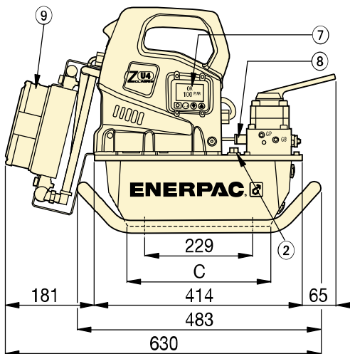
ZU4-Series with 4 and 8 litres reservoirs
