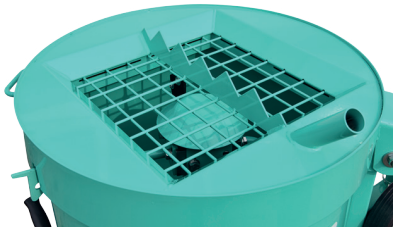
I-DUST grid with connection for vacuum cleaner: limits the dust in the surrounding environment.
