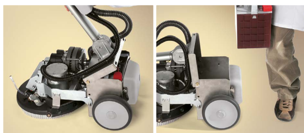
Vispa 35 B - Bs The battery compartment is easily accessible for quick battery replacement
