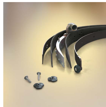
Vispa 35 E-B-BS In order to ensure excellent drying performance, the squeegee rubbers should be kept always clean. When worn out, they are very easy to replace
