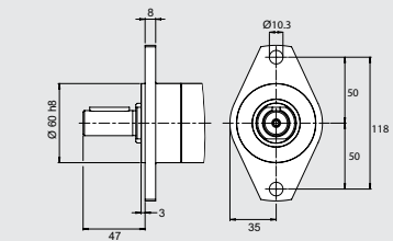
Stainless steel Flange Ordering No. 4430 2357 80
