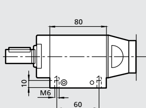
Foot Ordering No. 4430 0178 81
