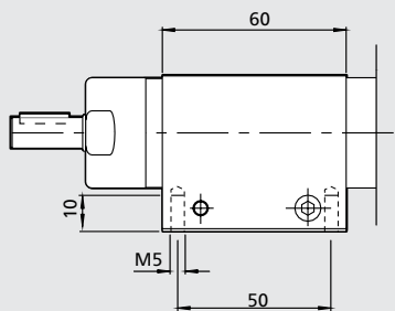
Foot Ordering No. 4430 0862 80
