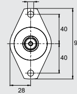
Stainless steel Flange Ordering No. 4430 1483 80
